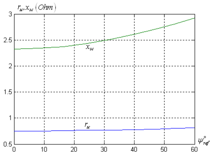
Fig.4.Characteristics of active ( r_{sc} ) and reactive ( x_{sc} ) components of impedance ( Z_{sc} ) for the short circuit mode of PST.
