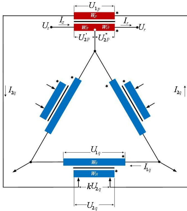
Fig.2. Traditional variant of PST (Marcerau Connection)
