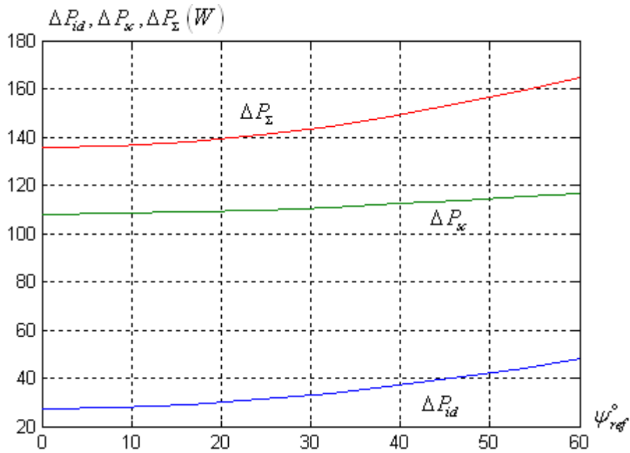
Fig.5. Nature of the change of power losses versus the angle \psi in the PST of Marcerau Connection.
